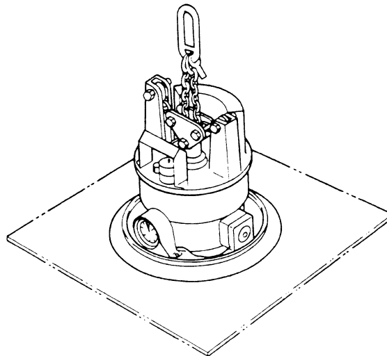
(b) Single-Pad Mechanical Vacuum Lifter
