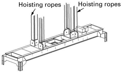
(a)(1) Lifting Beam (Hoisting Ropes)
