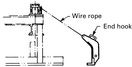
(m) End Hook, Spring-Type
