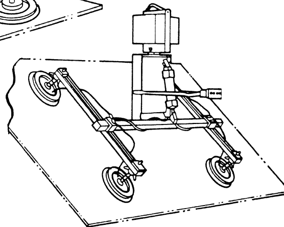
(e) Four-Pad Powered Vacuum Lifter Manipulator
