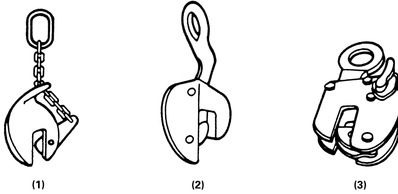
(a) Plate Clamps
