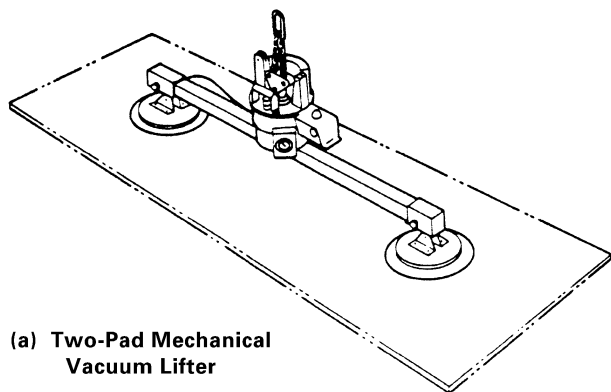
Fig. 20-0.4-1 Vacuum Lifters
