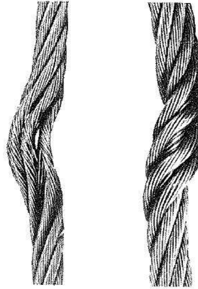
Figure 30-1.8.2-1 Distortion of Rope Structure — Kink
