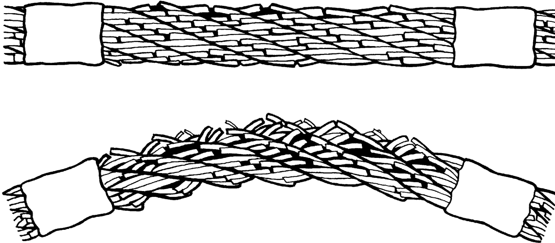
Figure 30-0.2-2 Crown Breaks
