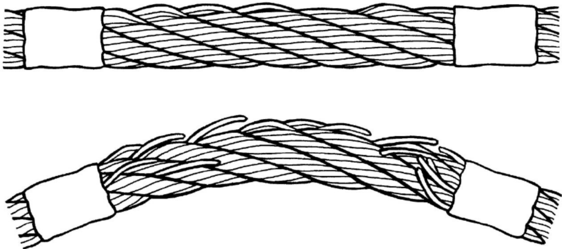
Figure 30-0.2-7 Valley Breaks
