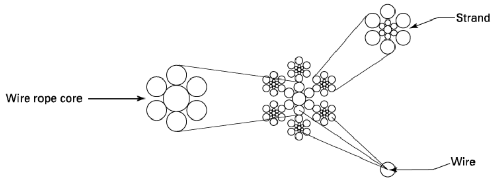
Figure 30-0.2-8 Wire Rope
