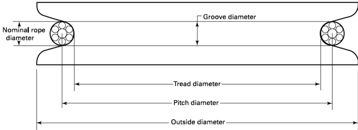
Figure 30-0.2-3 D/d Ratio
