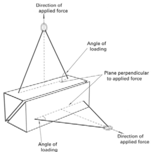
Fig. 9-2.5-1 Angle of Loading
