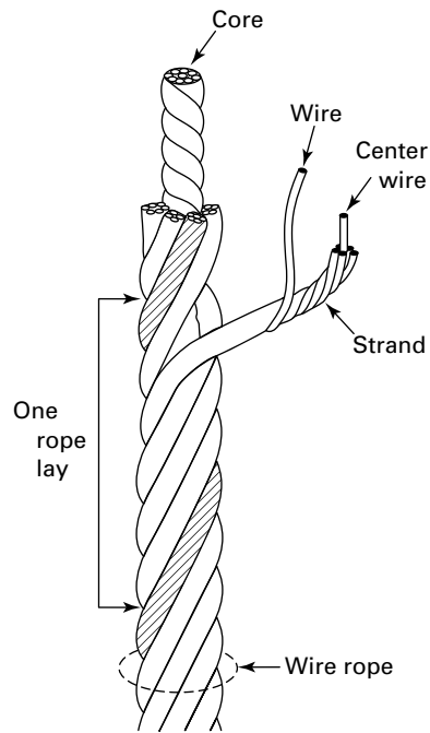
Fig. 9-2.0-2 Wire Rope
