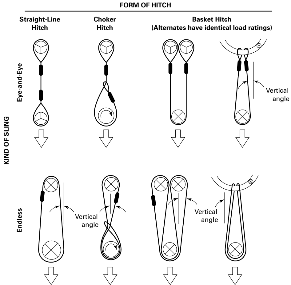
Fig. 9-4.5-1 Hitch Types for Synthetic Rope Slings
